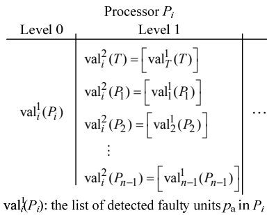
Fig. 5 The FG-tree stored in processor P_i for two levels ( T =source processor)
