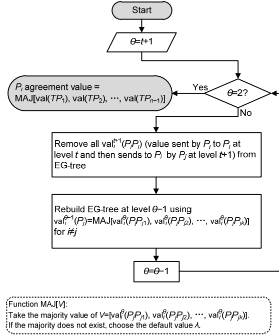
Fig. 4 Finding the Byzantine agreement value in fault-free processor P_i ( T =source processor and MAJ is the majority function)
