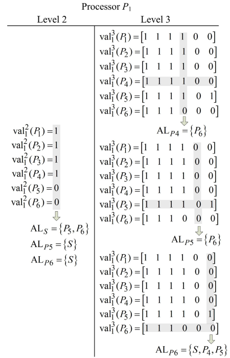
Fig. 8 Local fault diagnosis in processor P_1 during the Byzantine agreement process
