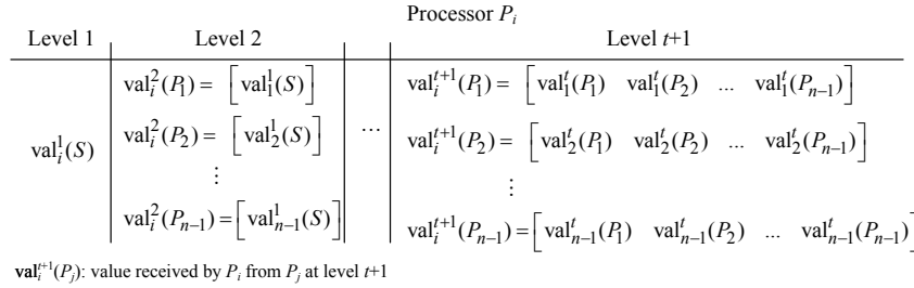
Fig. 2 A (t+1) -level EG-tree of processor P_i in Fig. 1
