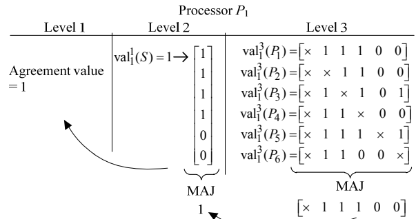
Fig. 9 Decision-making phase to find the Byzantine agreement value in processor P_1
