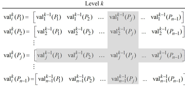
Fig. 3 Level k of the EG-tree stored in processor P_i (The shaded area is used to check the faulty status of P_j )
