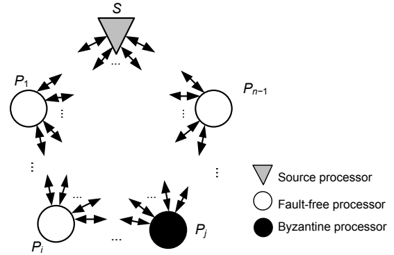
Fig. 1 A fully connected network with n processors and \lfloor (n-1)/3 \rfloor faulty processors
